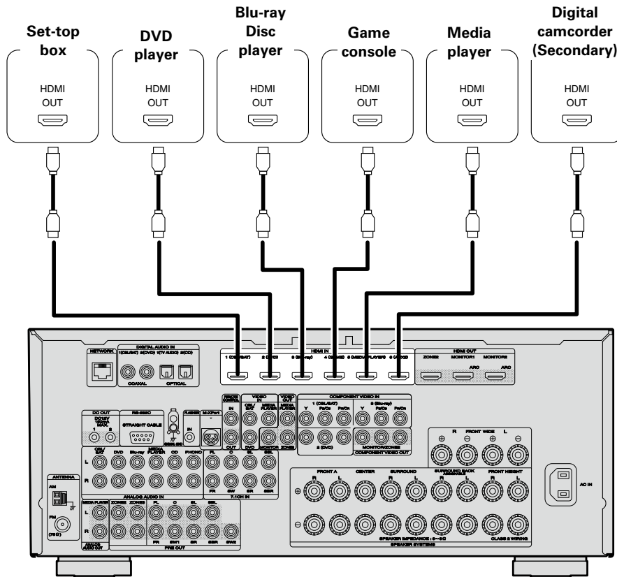
[Rear panel]
